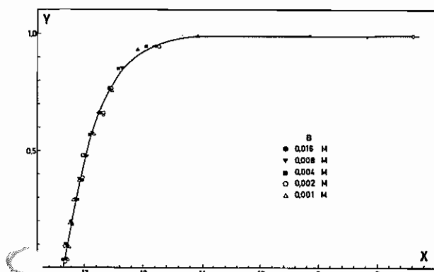
Figure 4. The Y, X curve of the system nickel(II) and 3-mercaptopropanediol.
