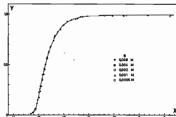
Figure 3. The Y, X curve of the system nickel(II) and 2-mercaptoethanol.
