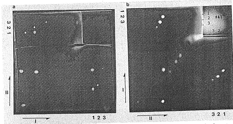
Fig. 5. (a) Two-dimensional thin-layer chromatogram on silica gel 60 (10 × 10 cm) of a fat extract contaminated with 1 ppb DES. Starting point overspotted with 2.5 ng DES before development in second direction. References in side lanes: 1 = 2.5 ng DES; 2 = 10 ng 17β-estradiol; 3 = 20 ng oestrone. Developing solvents: I = chloroform-ethanol-benzene (36:1:4); II = n -hexane-dichloromethane (4:3:2). (b) Two-dimensional thin-layer chromatogram on silica gel 60 (10 × 10 cm) of a fat extract contaminated with 2 ppb 17α-methyltestosterone. Starting point overspotted with 3 ng 17α-methyltestosterone before development in second direction. References in side lanes: 1 = 3 ng 17α-methyltestosterone; 2 = 3 ng testosterone; 3 = 2 ng trenbolone. Developing solvents: I = chloroform-methanol-benzene (36:1:4); II = n -hexane-dichloromethane-ethyl acetate (1:2:2).
