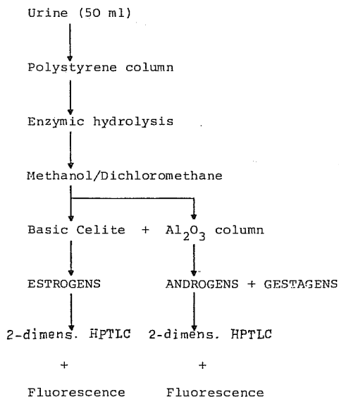
Fig. 2. Scheme for detection of anabolic steroids in urine.
