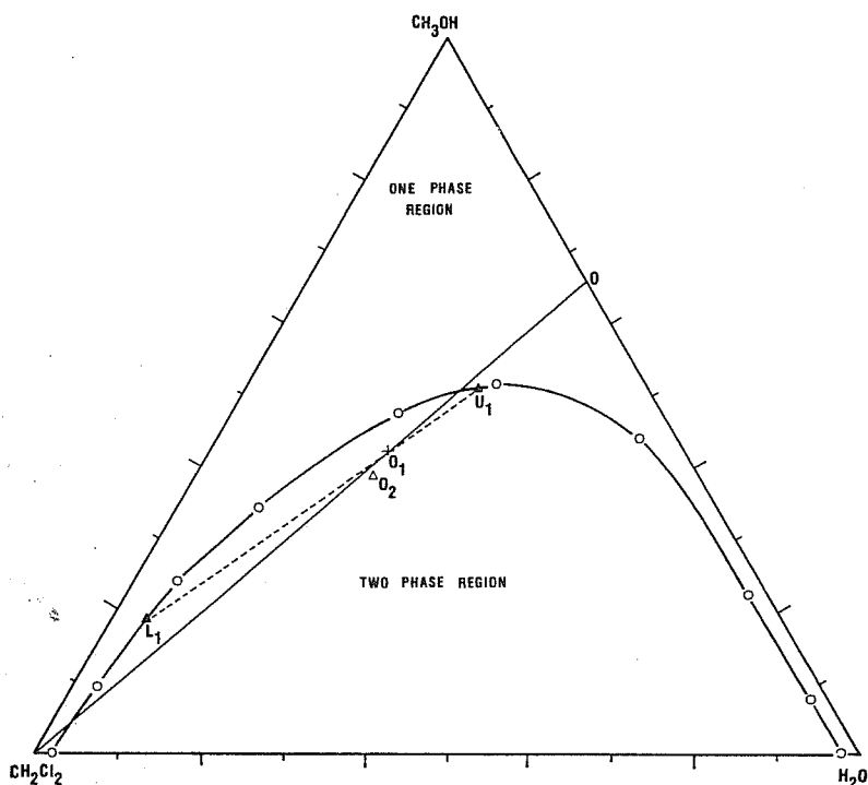
Fig. 4. Ternary liquid-liquid miscibility diagram of dichloromethane-methanol-water at ambient temperature (20°).
