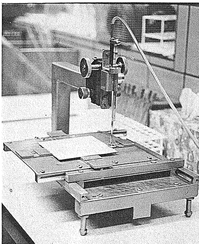
Fig. 3. Spot applicator for dispensing sample volumes at the nanolitre level.
