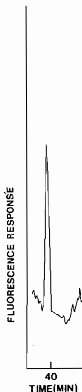
Fig. 4. Chromatogram after post-column derivatisation of 10 ng of DES.
