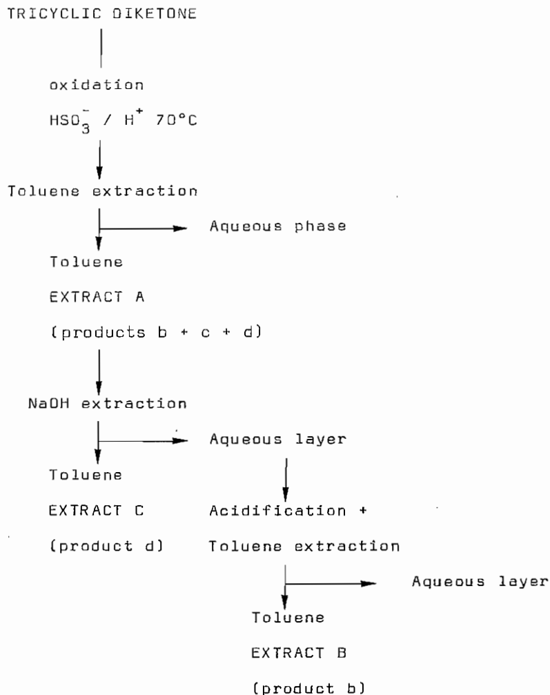
Fig. 3. Extraction scheme for the isolation of the oxidation products of phenanthrenedione.
