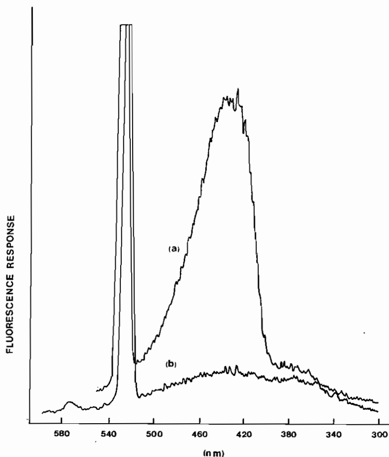
Fig. 8. Emission spectrum ( \lambda_{\text{exc.}} = 260 nm) of a neutralized reaction mixture after irradiation and subsequent conversion with hydrogen sulphite: (a) 0.180 ng/ml DES; (b) blank.
